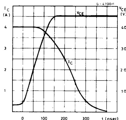
Figure 6. Turn-off Phase.
